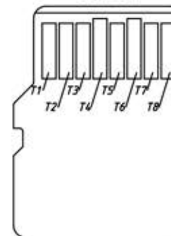
micro SD card back view
