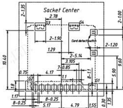
RECOMENDED PCB LAYOUT TOLERANCK:±0.05
